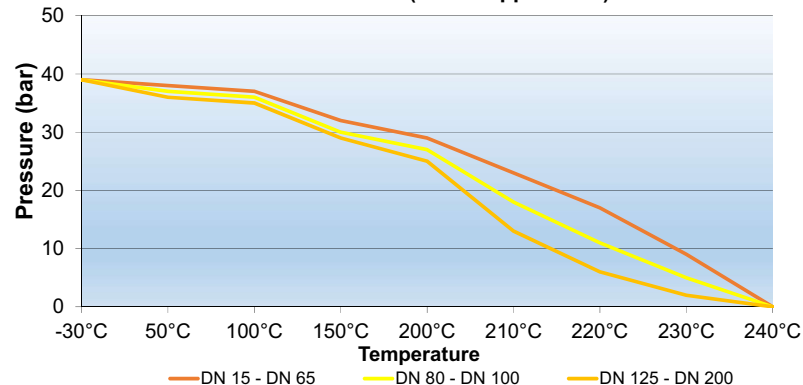
Pressure - Temperature Diagram Ball seal TFM4215 (Steam application)
