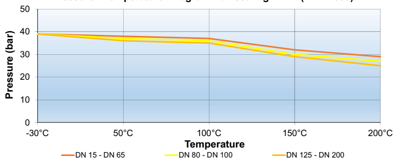
Pressure - Temperature Diagram Ball sealing PTFE (TFM-1600)
